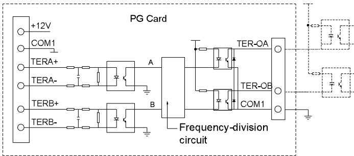
Figure 7.12 Wiring Diagram of PG Card Frequency-division Output.
