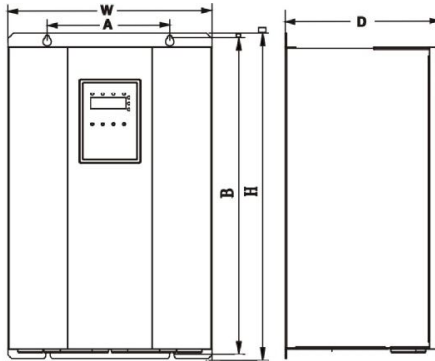
Figure B.2 Dimensions (18.5~30kW).
