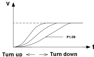
Figure 6.4 S - curve setting sketch map description.
